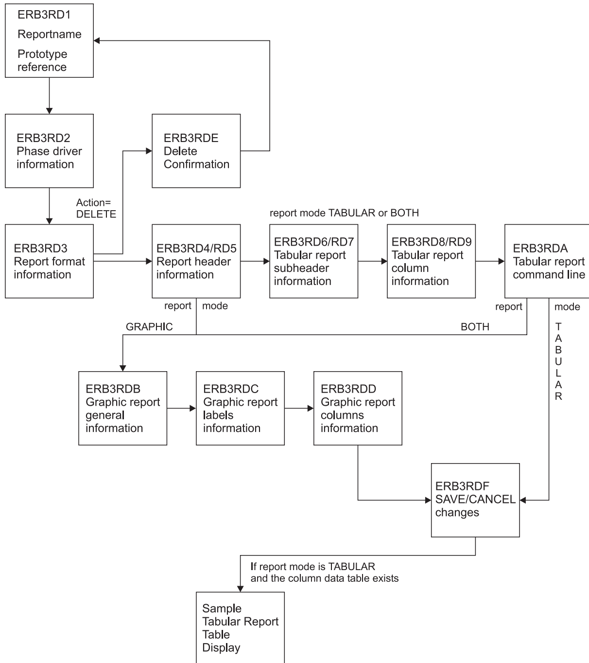
Figure 25. Panel Sequence for the Report Definition Utility
