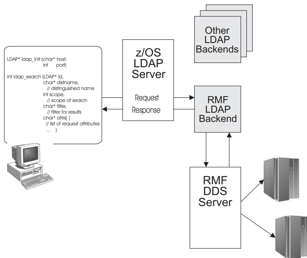
Figure 7. Accessing Performance Data from LDAP
