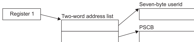
Figure 46. ERB3SOCK Input Parameter Structure
