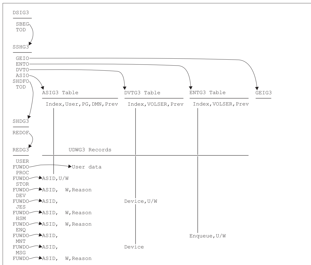
Figure 48. Monitor III Measurement Table and Record Relationships
