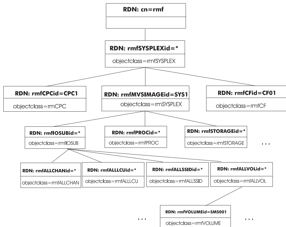
Figure 6. Sample DIT Portion of the RMF LDAP Performance Data
